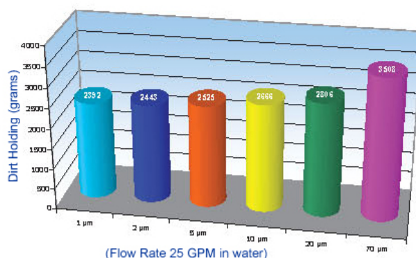
Poliflo BF - Size # 2 Dirt Holding (grams)
